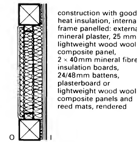
8 New panel
